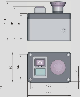
Snap-in mounting 安装孔尺寸
