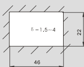
Snap-in mounting 安装孔尺寸
